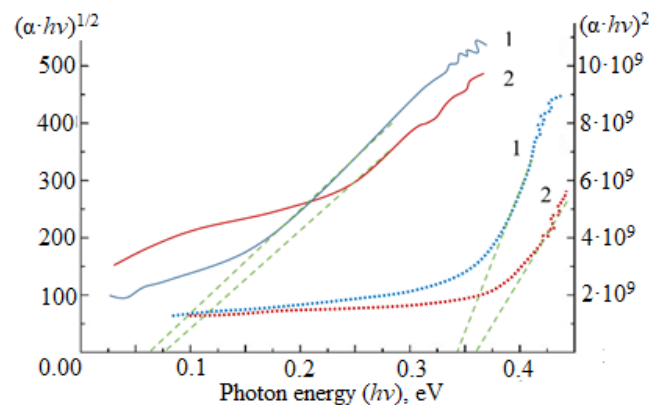
Figure 10. Tauc diagrams for indirect and direct band gaps of amorphous (sputtered) and nanostructured (annealed) \text{CrSi}_2 thin films.
