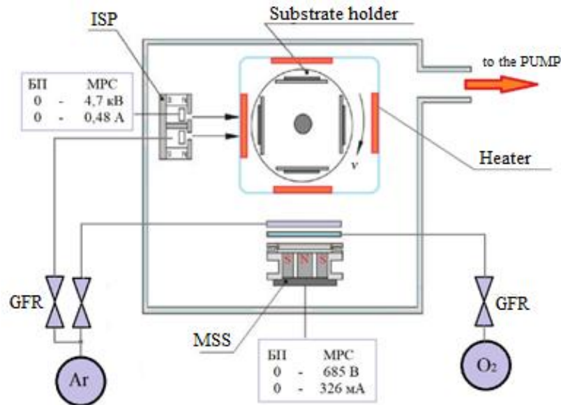
Figure 1. Diagram of the experimental setup for the formation of a \text{CrSi}_2 film by the solid-phase ion-plasma method: ISP - ion source for purification, MSS - magnetron sputtering system, GFR - gas flow regulator
