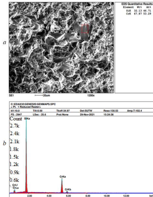
Figure 2. Results of studying the \text{CrSi}_2 target using a scanning electron microscope: SEM image of the surface (a) and EDX spectrum (b)
